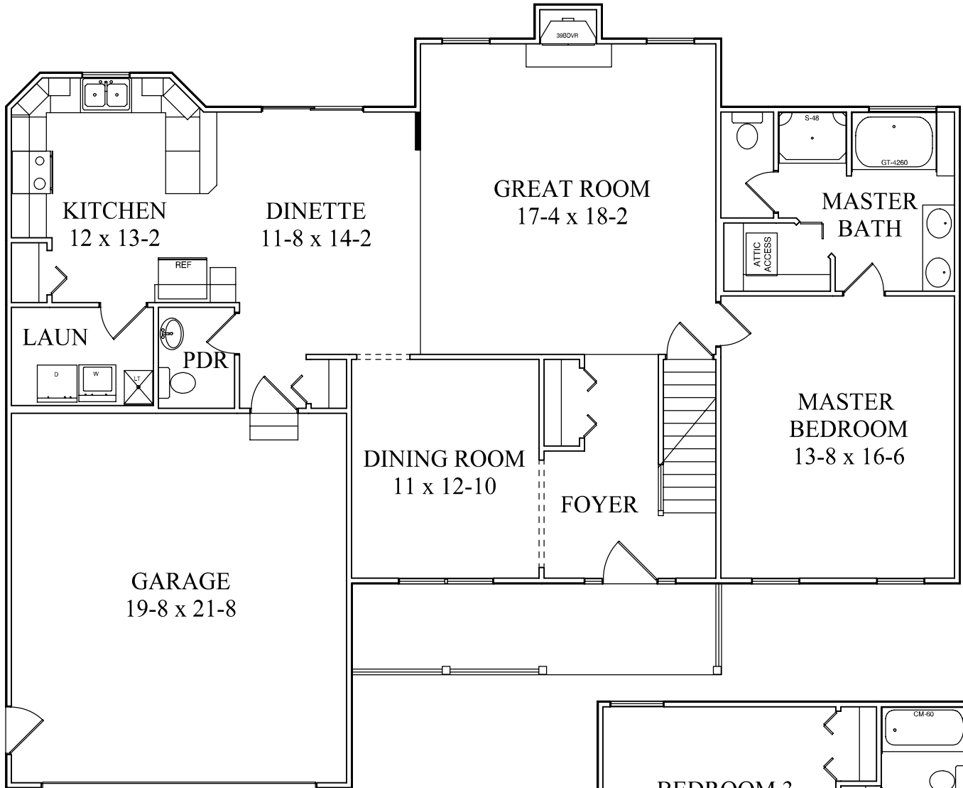
First Floor Plan 1460 Square Feet
