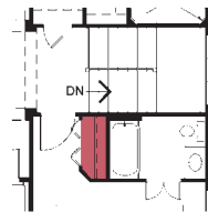
Suite 2 15'0" x 14'4" optional basement stair location
